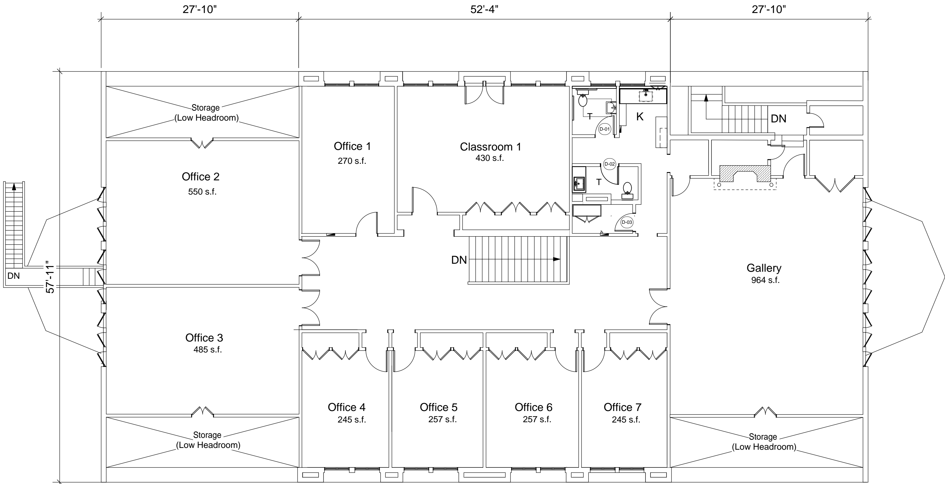
Haver Hall Second Floor Plan
